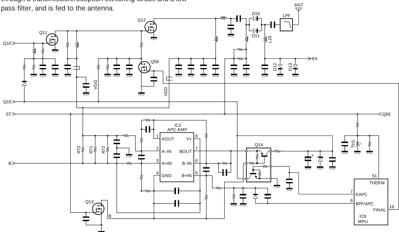
Fig. 7 APC and Temperature protection circuit
